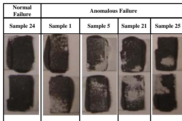
Fig. 3 Post-test fracture surfaces: Sample 24 is the sample identified in Table 5 as EBX-24. Samples 1, 5, 21, and 25 are the starred samples in Table 4 and all exhibited low fracture shear stresses
